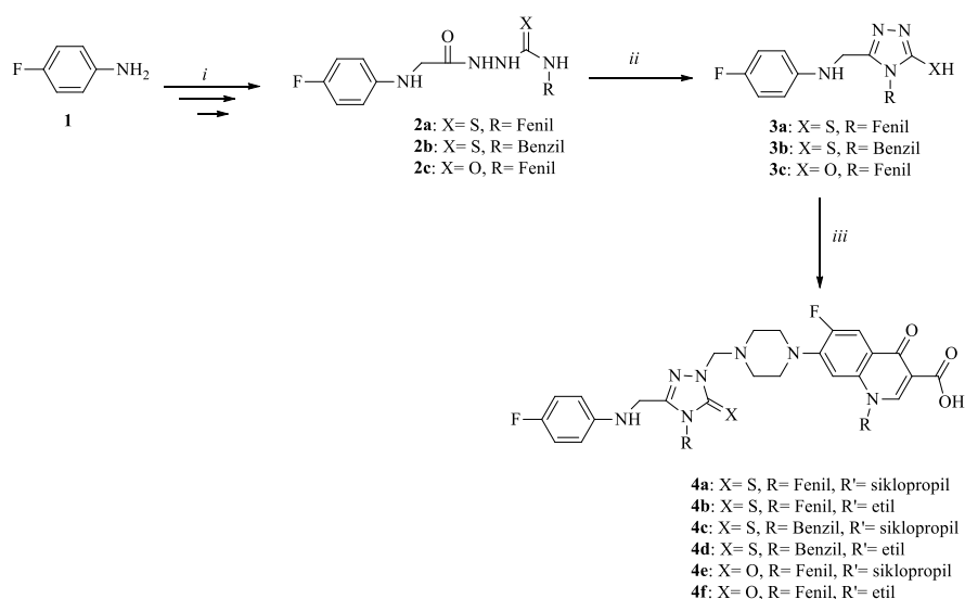
Scheme 1: i : Ethyl bromoacetate, THF; Hydrazine hydrate, Ethanol, Aryl iso(thio)cyanoate, Ethanol, ii : NaOH, H 2 O/Ethanol, iii : DMF, Formaldehyde, Norfloxacin or Ciprofloxacin
