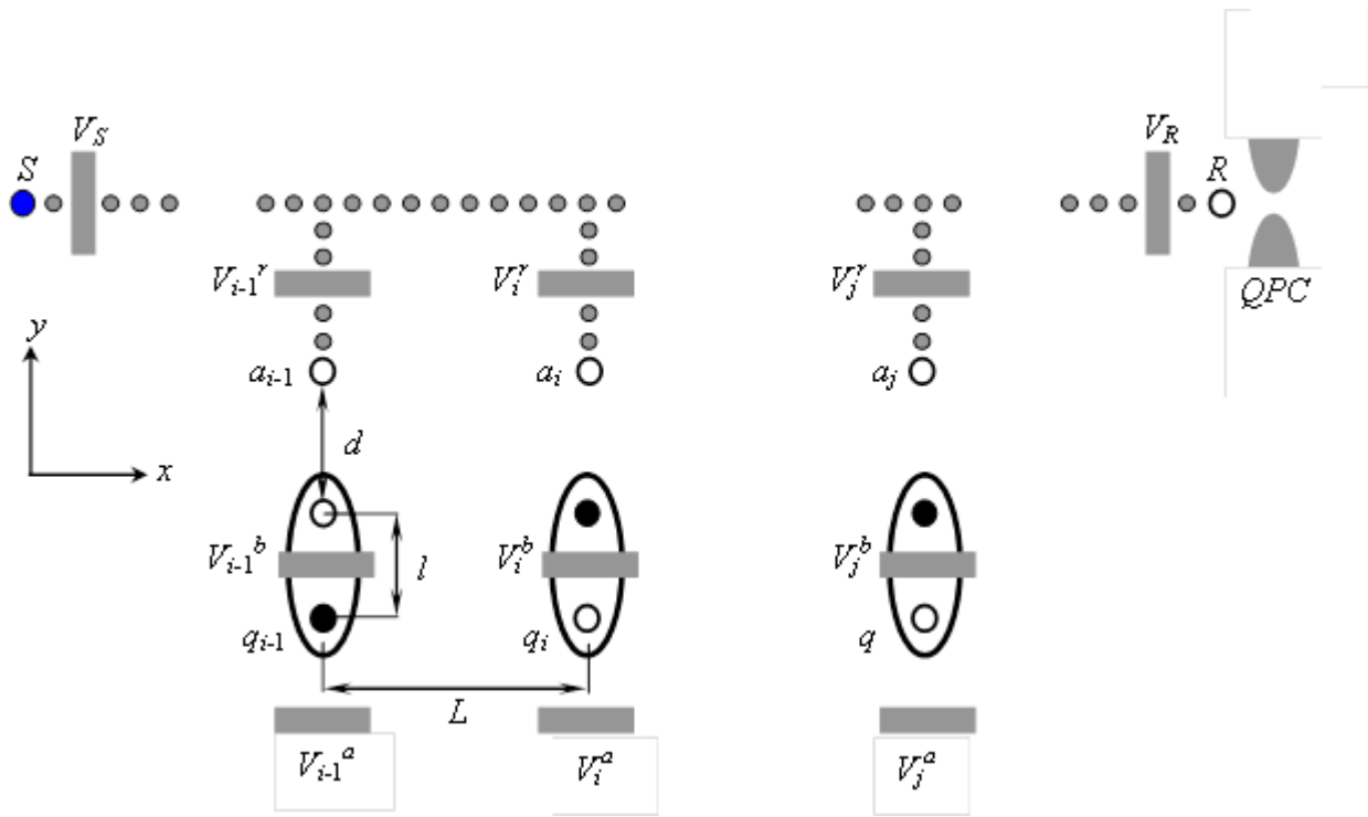
Fig. 7. Schematic diagram of a full-scale quantum computer. Each qubit q_i , i=1 - is equipped with auxiliary gates V_{i-1}^a , V_i^b and V_i^r . The filled (empty) circle symbolizes a donor with (not containing) a localized electron in the ground state. The auxiliary structure is formed from quasi-linear chains of ionized donors, at the ends of which are auxiliary donors S , R and a_i , and contains a localized probe electron in the ground state of the donor S . The set of gates V_S , V_R and V_i^r is used to create an effective optical tunneling channel that provides indirect interaction of an arbitrary pair of qubits.
